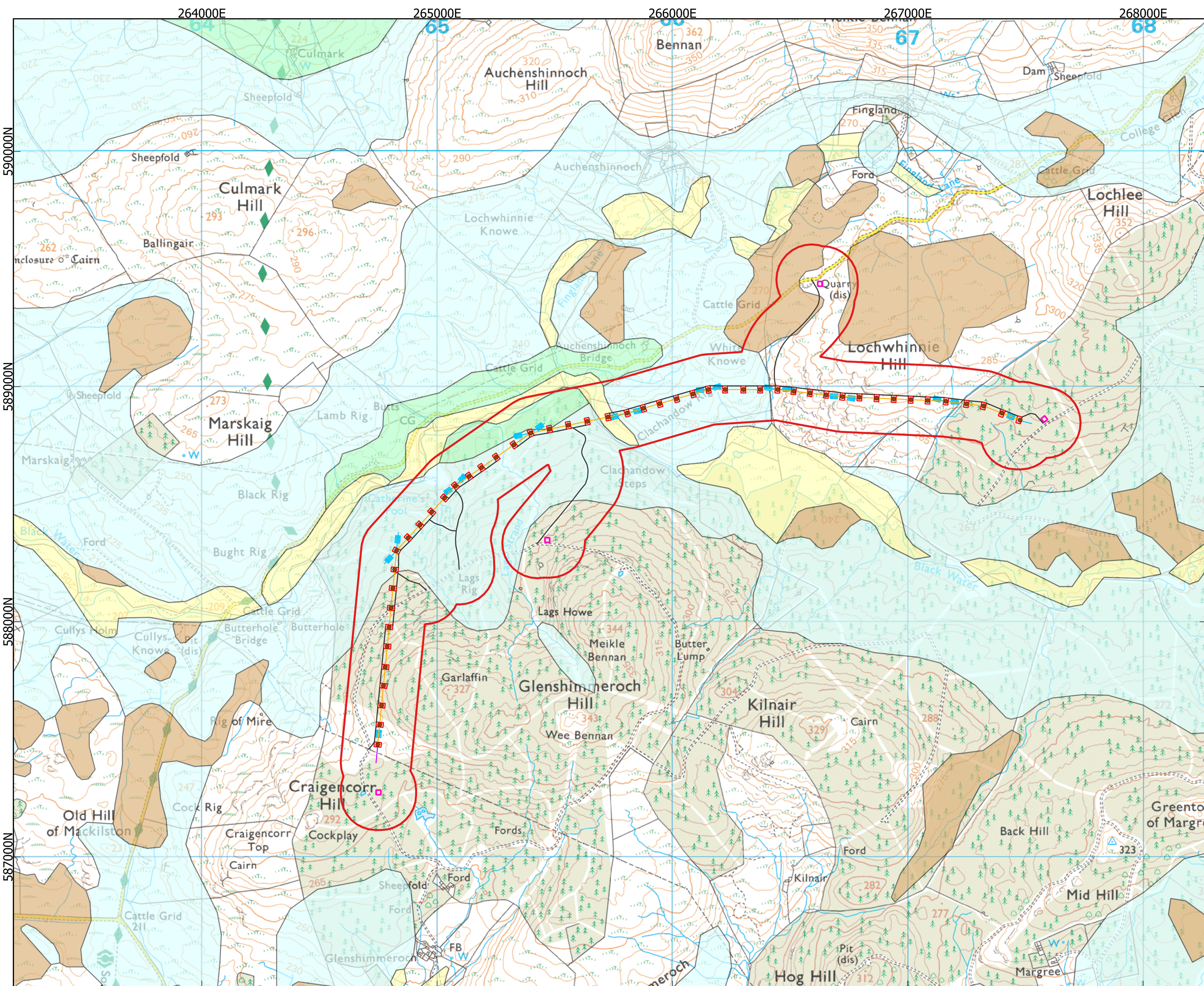
TITLE: Figure 9.3: Superficial Geology
