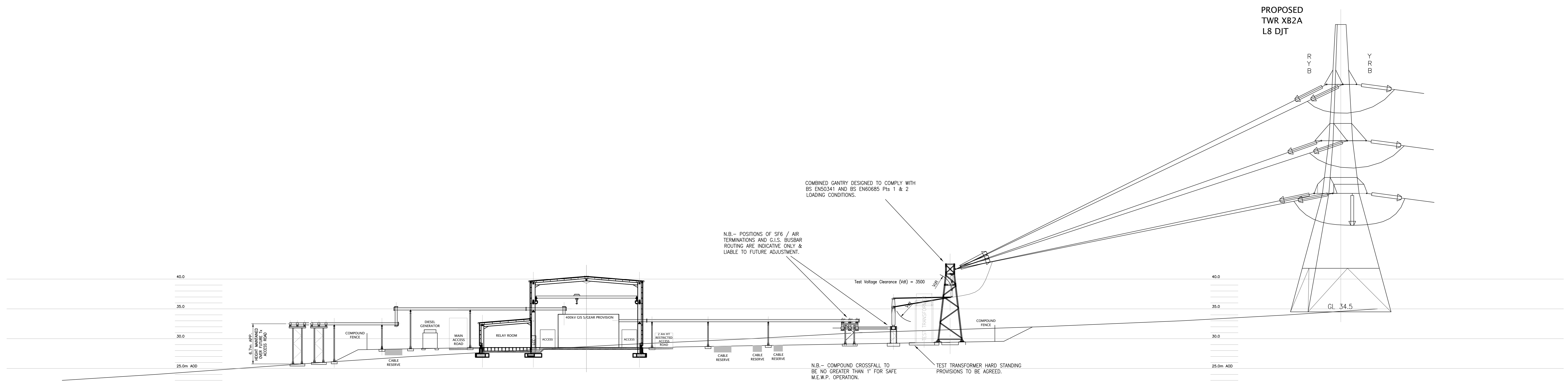
ELEVATION SHOWING PROPOSED TOWER XB002A
