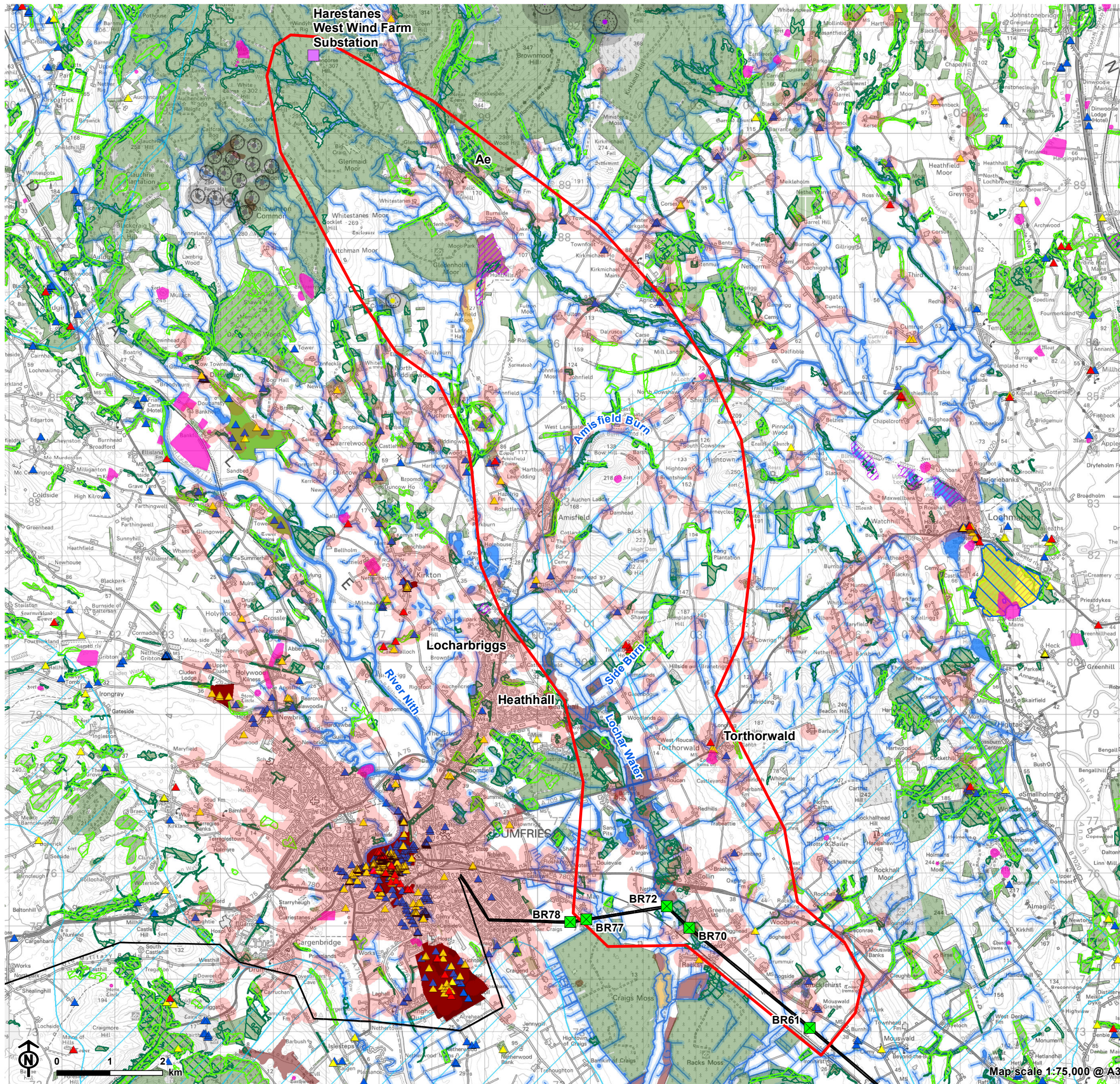
Figure 4.2: Routeing Considerations
