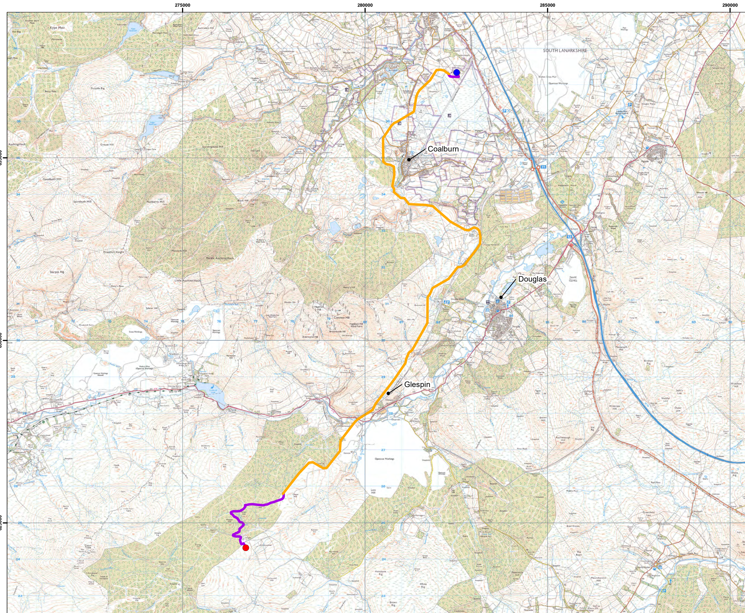
TITLE: Figure 1.1: Kennoxhead Wind Farm to Coalburn Substation Overhead Line – Overview
